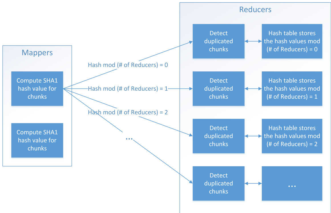
Figure 3.4. Map-Reduce structure
